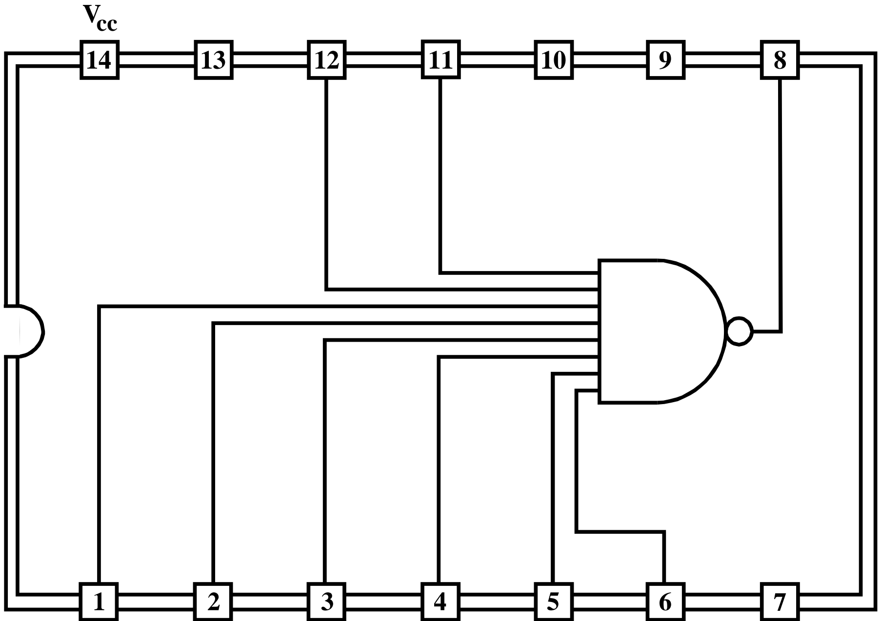
7430: 8-INPUT NAND
