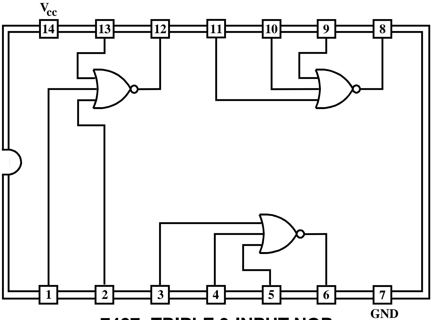
7427: TRIPLE 3-INPUT NOR
