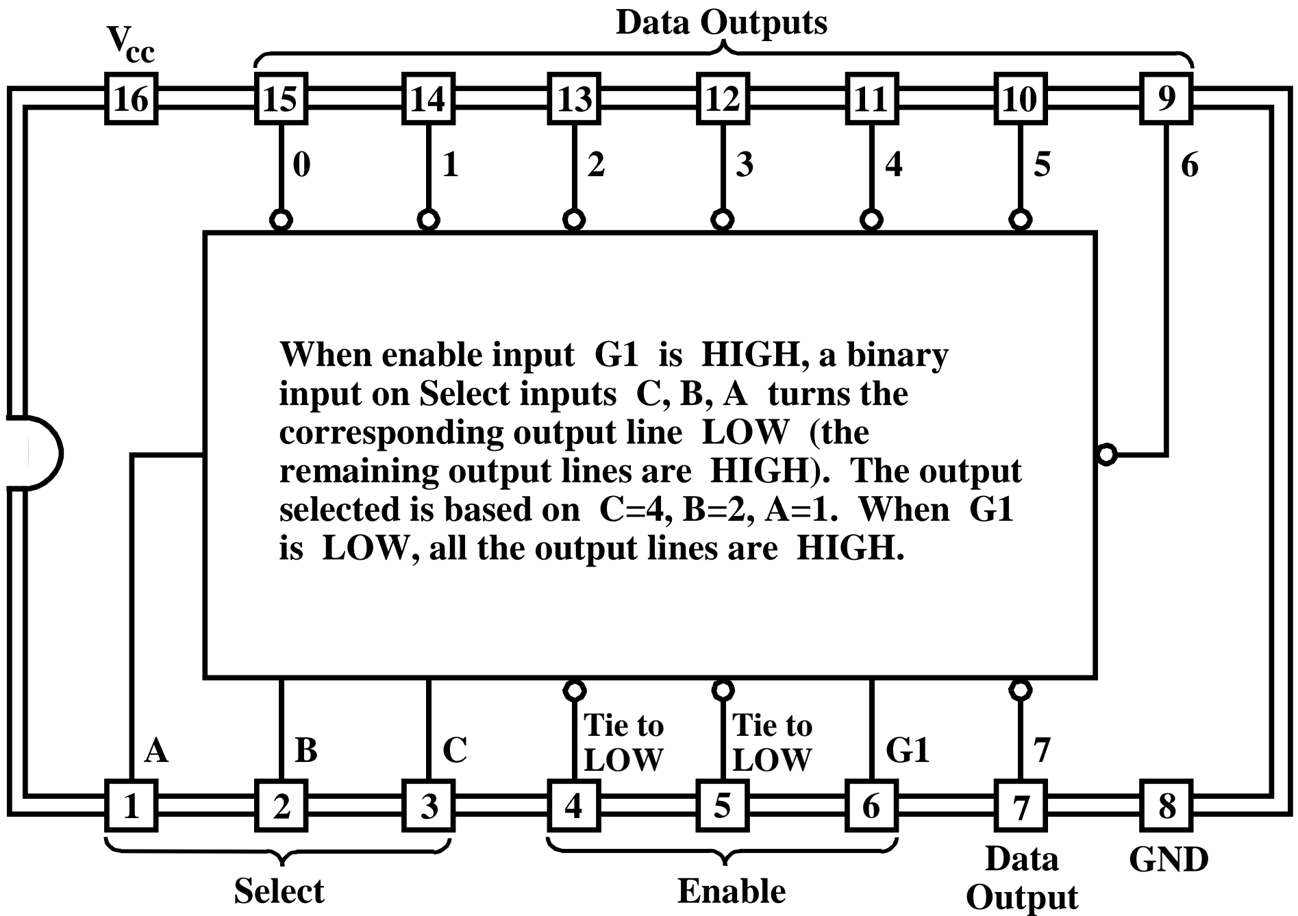
74138: 3 TO 8 DECODER/DEMULTIPLEXER
