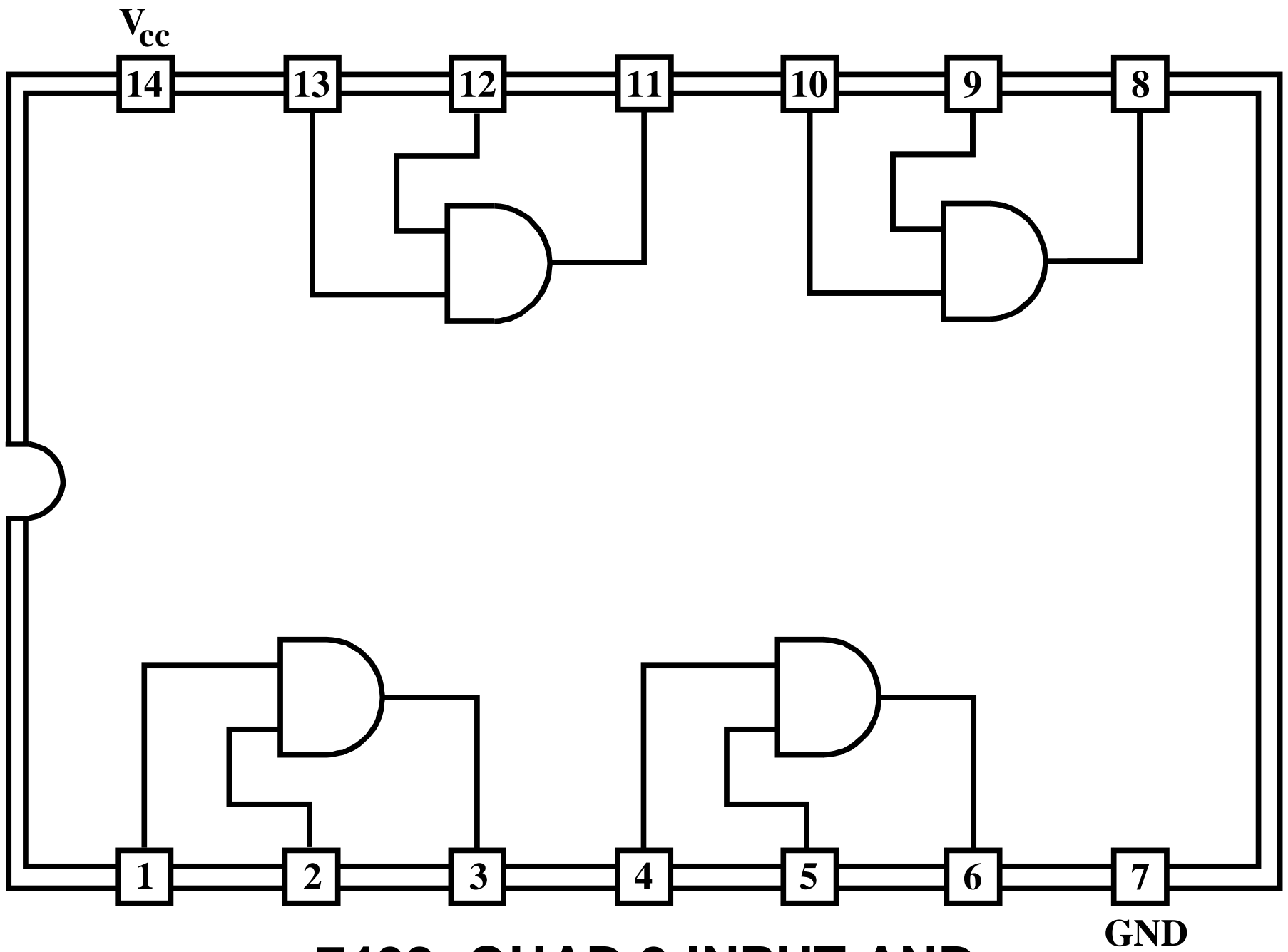
7408: QUAD 2-INPUT AND
