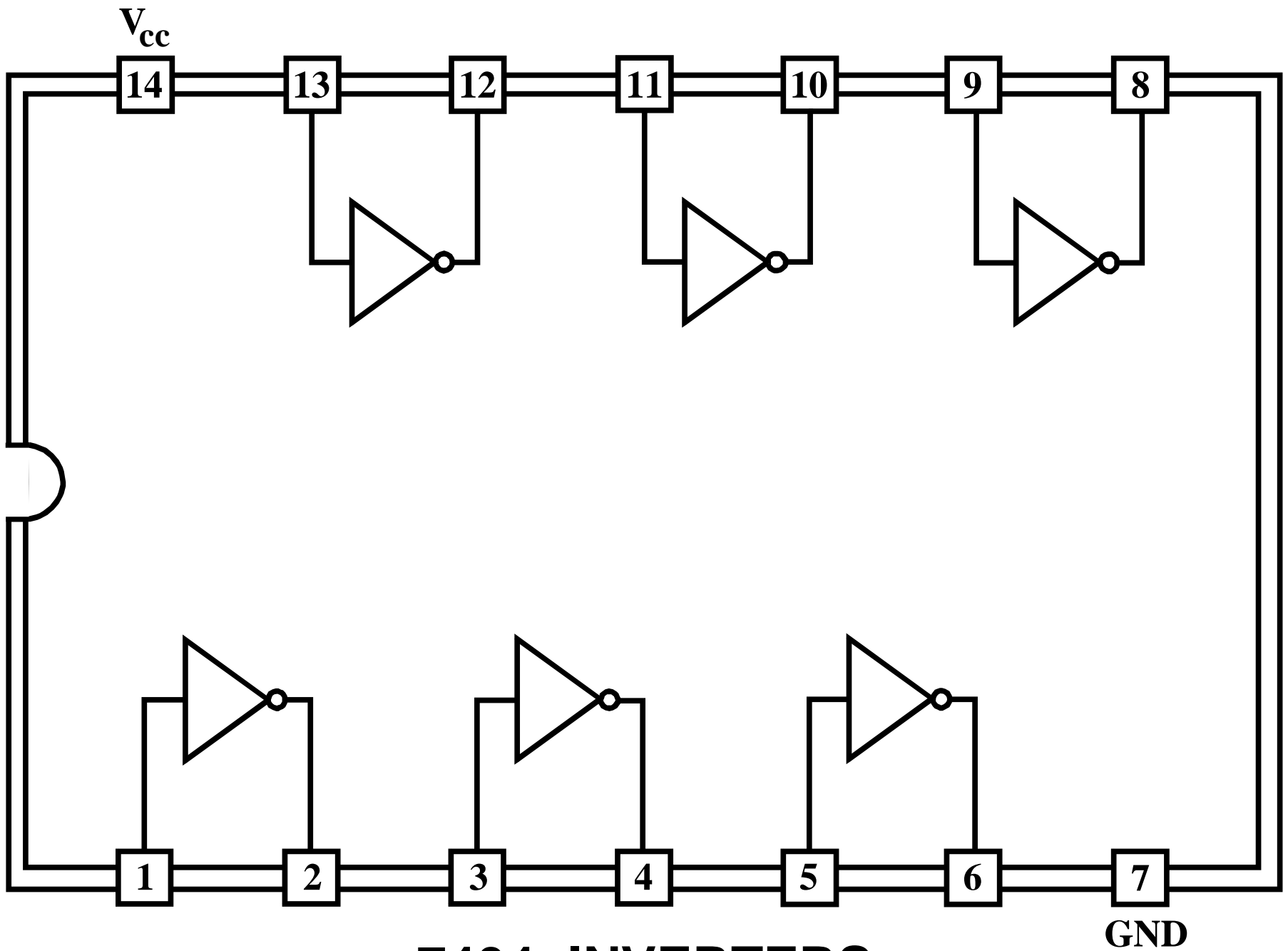
7404: INVERTERS
