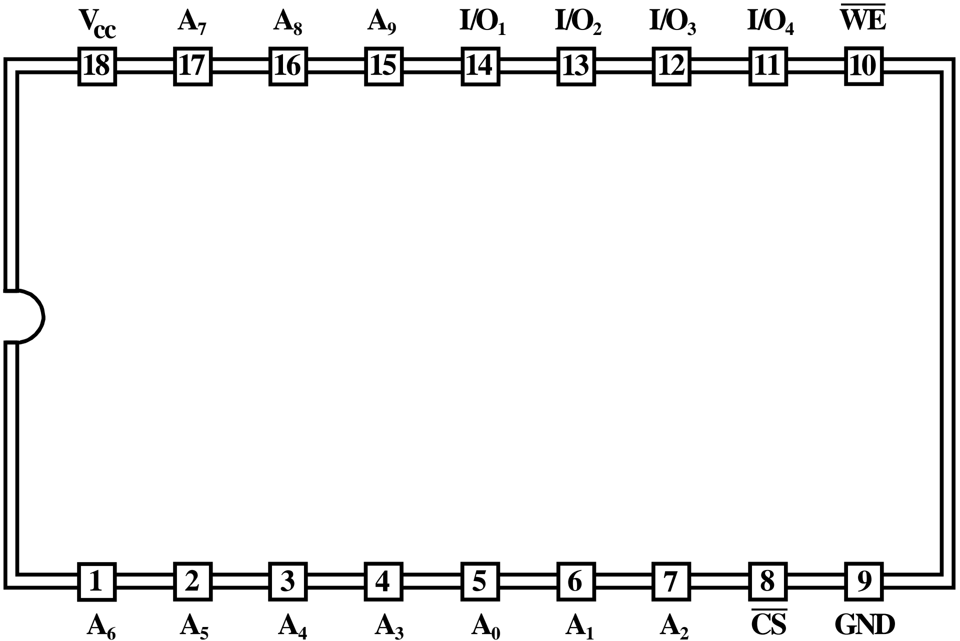
2114: 1K x 4-BIT STATIC RAM - V_{cc} = +5V
